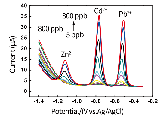
Stripping voltammetric curves in the solution dissolved with \text{Pb}^{2+} , \text{Cd}^{2+} , and \text{Zn}^{2+} ions
