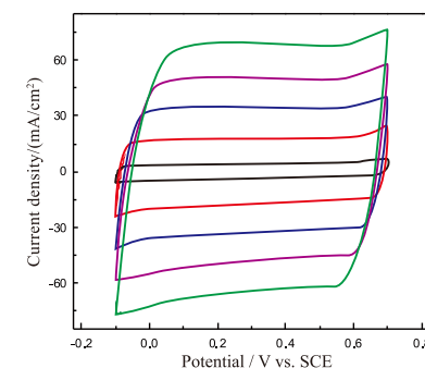
CV of PPY supercapacitor in 0.5 mol/L \text{H}_2\text{SO}_4 solution
